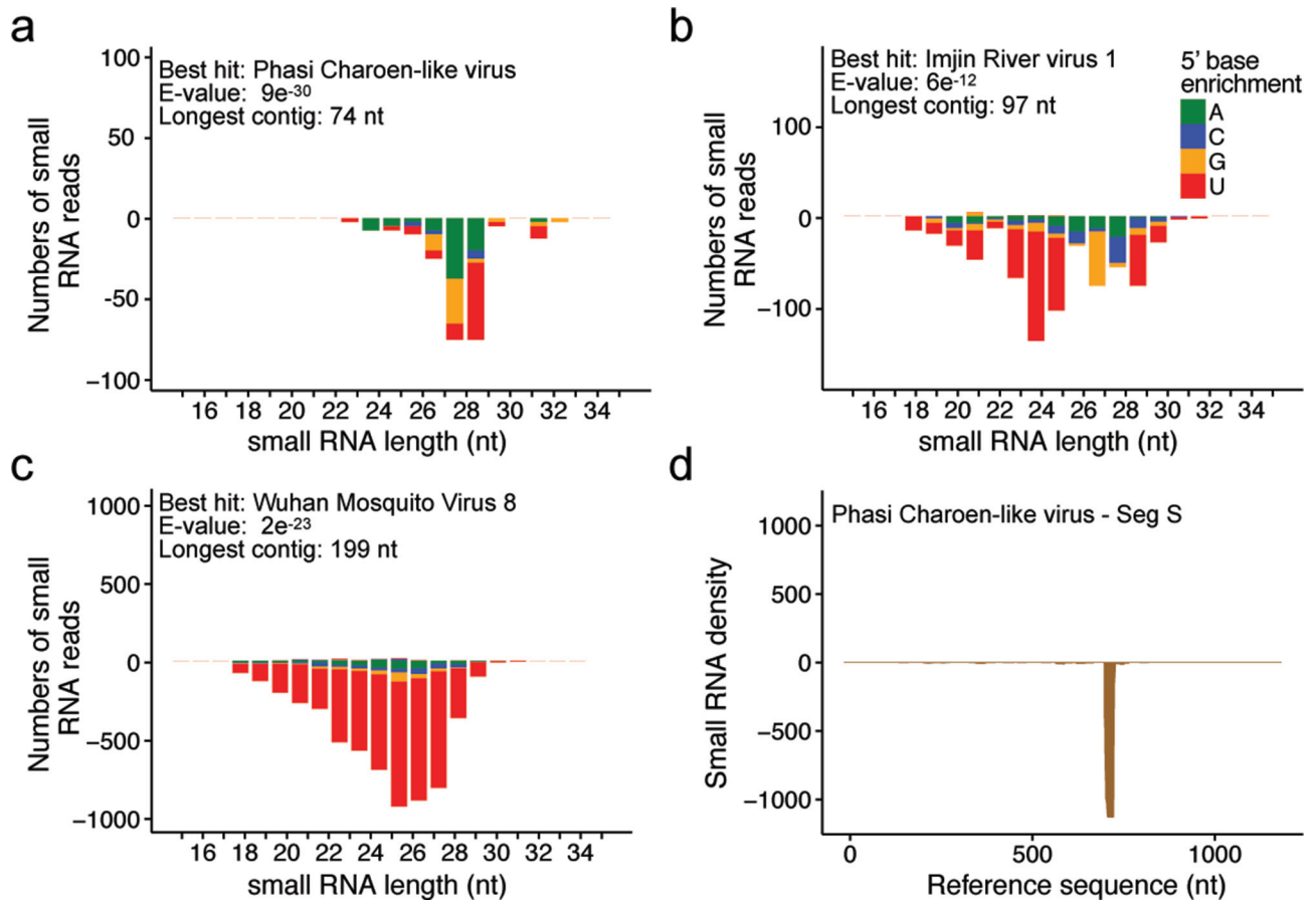
Fig. 3. Small RNA size profiles of endogenous viral elements (EVEs) found in Cx. quinquefasciatus mosquitoes. (a–c) Size distribution of small RNAs originating from EVEs that showed similarity to PCLV (a), IRV1 (b) and WMV (c). (d) Density of small RNAs aligned to the S segment of PCLV. E-value and contig size are shown. 5' Base preferences of small RNAs are indicated by colour.
