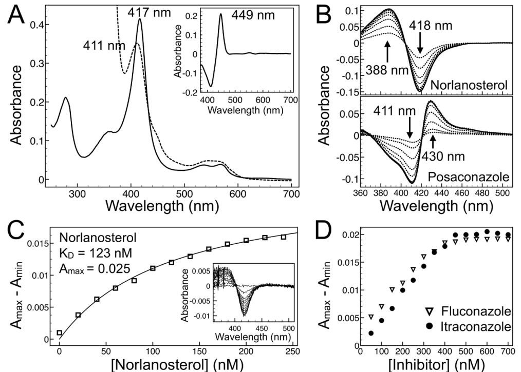
Fig 6. Spectroscopic analysis of recombinant NfCYP51. (A) Absolute UV-visible spectra of 3.5 \mu\text{M} purified recombinant NfCYP51: ferric, \text{Fe}^{3+} ,—solid line, ferrous, \text{Fe}^{2+} ,—dashed line. Inset: \text{Fe}^{2+} - \text{Fe}^{2+}\text{CO} difference spectra. (B) Type I (31-norlanosterol) and type II (posaconazole) difference spectra both added in 500 nM increments to 3.5 \mu\text{M} NfCYP51. (C) Binding isotherm of 31-norlanosterol added in 25 nM increments to 0.2 \mu\text{M} NfCYP51 and absorbance difference spectra (Inset). (D) Binding isotherms of posaconazole and fluconazole, both added in 50 nM increments to 0.5 \mu\text{M} NfCYP51, show a linear increase in signal up until the equivalence point, after which no further increase in signal was detected.
