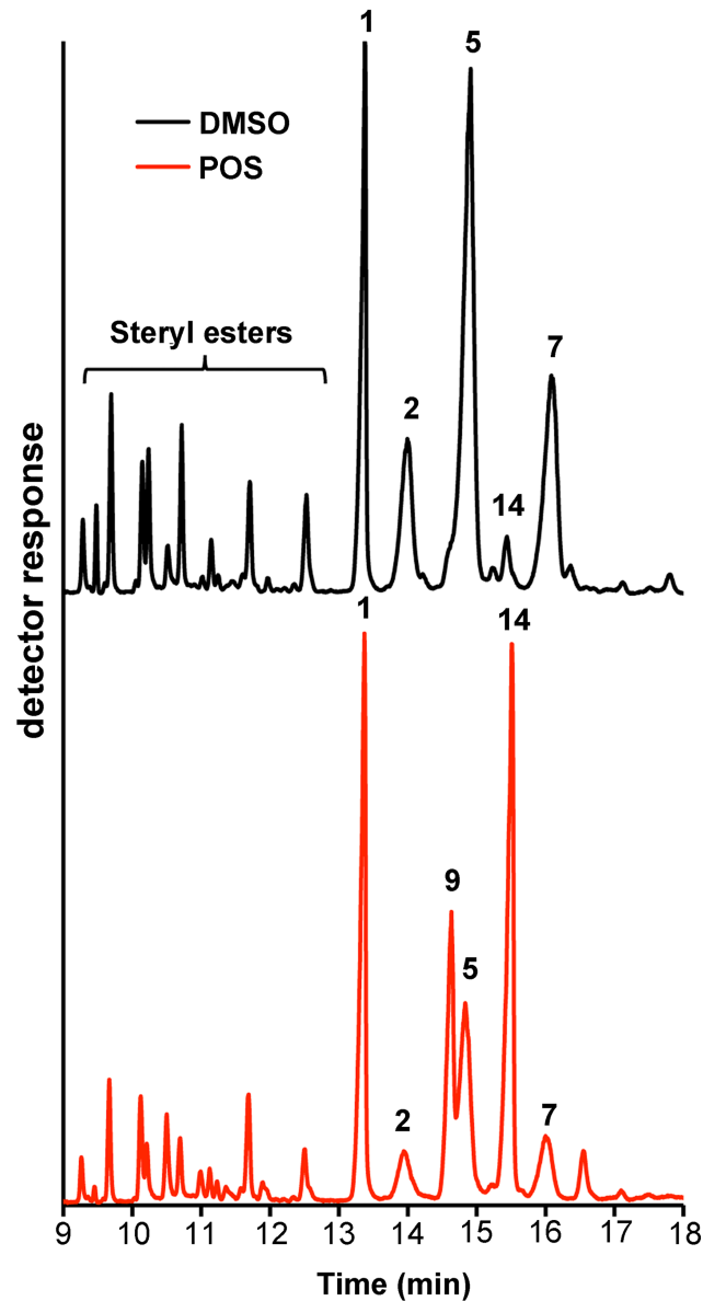
Fig 3. Gas chromatography separation of the total sterol fractions extracted from N. fowleri trophozoites. Chromatogram fragments from the non-derivatized DMSO- ( black trace ) and posaconazole (POS)-treated ( red trace ) sterol extracts are shown. Peaks are labeled according to Table 2 . The content of 31-norlanosterol ( 14 ) remarkably increased in posaconazole-treated samples.
