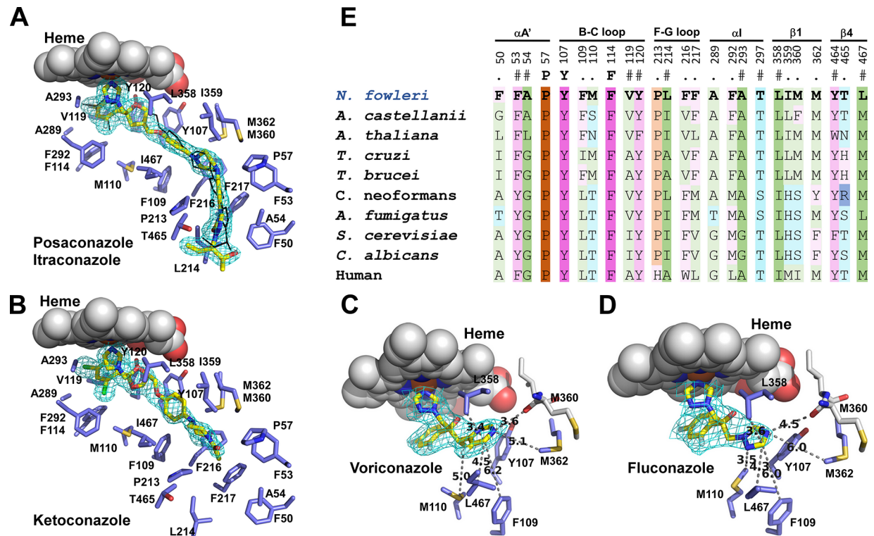
Fig 7. NfCYP51-inhibitor binding. (A) Posaconazole (yellow sticks) and itraconazole (black lines) are shown overlapped. Fragment of the 1.7 Å 2F_o - F_c electron density map countered at 1.0\sigma is shown for posaconazole (cyan mesh). Amino acid residues within 5 Å are in blue, heme is in spheres. Ketoconazole (B), voriconazole (C) and fluconazole (D) are shown in yellow sticks with the corresponding map fragments in cyan mesh. In C and D, amino acid contacts only for the inhibitor moiety distant from the heme macrocycle are shown. Distances are in Angstroms. (E) Amino acid residues within 5 Å of bound posaconazole in NfCYP51 (highlighted in bold) are propagated to the CYP51 sequences from the indicated species. Residue labeling is according to NfCYP51. Secondary structure elements on the top are labeled according to the nomenclature introduced elsewhere.[47] The color scheme is according to the side chains: hydrophilic neutral (cyan), aromatic (purple), hydrophobic (green) and proline (ochre). Residue conservation is indicated by the color shades, with pale → bright gradient corresponds to conservation levels. Invariant positions are in brightest shades.
