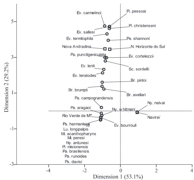
Fig. 2. Results of correspondence analysis among the phebptomine species and the municipalities of Nivarai, Nova Andradina, Novo Horizonte do Sul and Rio Verde de Mato Grosso from July 2008 to June 2010. (■) Municipality, (●) species.
