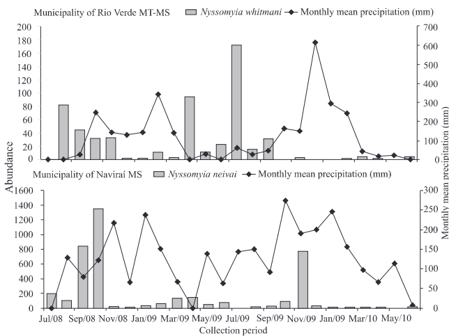
Fig. 1. Monthly variation of the abundance of Nyssomyia whitmani and Nyssomyia neivai in relation to the monthly mean precipitation in Rio Verde de Mato Grosso and Nivarai municipalities, from July 2008 to June 2010.
