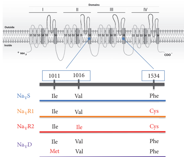
FIGURE 1: Voltage gated sodium channel (Na V ) kdr alleles of Aedes aegypti populations from Brazil. Schematic representation of the Na V , with its four domains, each with six hydrophobic segments. The kdr sites 1011 and 1016 are in the IIS6 segment, while the 1534 site lies in the IIIS6. Each haplotype is represented by means of the variation at each kdr site, where wild-type and kdr aminoacids are indicated in black and red, respectively. The colours of the alleles are the same in the following figures.
