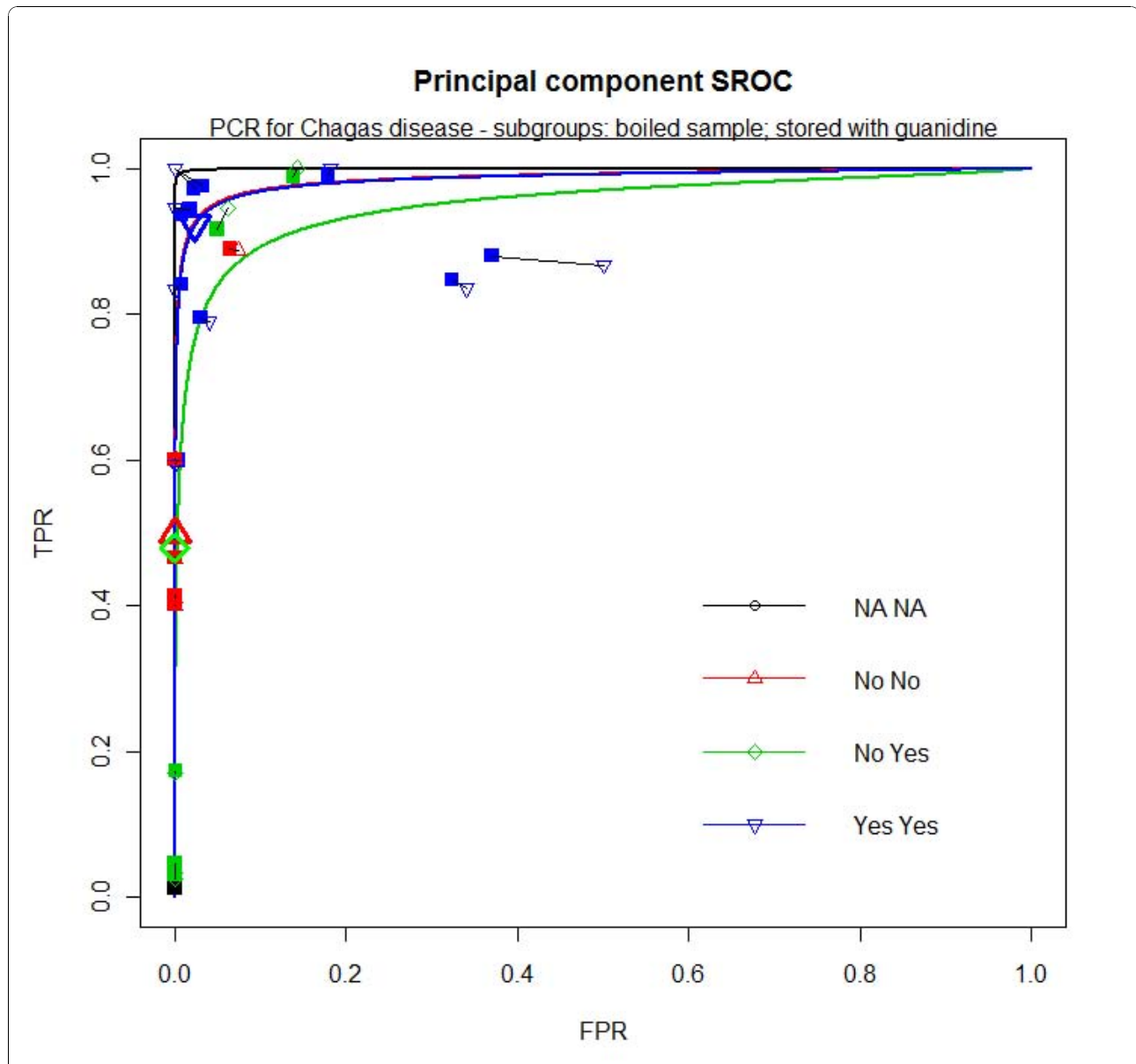
Figure 5 PCR for Chagas disease HSROC - subgroups of blood samples boiled before processed and stored with guanidine. Big blue upside down triangle - summary estimate of the group stored with guanidine and boiled; Big green diamond - summary estimate of the group stored with guanidine and not boiled; Big red triangle - summary estimate of the group not stored with guanidine and not boiled; Blue small squares and blue small upside down triangles - shrunken estimates from bivariate model and crude estimates (respectively) from group stored with guanidine and not boiled; blue solid line - SROC curve from group stored with guanidine and boiled; dot - crude estimates; small green squares and small green diamonds - shrunken estimates from bivariate model and crude estimates (respectively) from group stored with guanidine and not boiled; solid green line - SROC curve from group stored with guanidine and not boiled; small red squares and small red triangles - shrunken estimates from bivariate model and crude estimates (respectively) from group not stored with guanidine and not boiled; red solid line - SROC curve from group not stored with guanidine and not boiled; NA - not assigned or missing.
