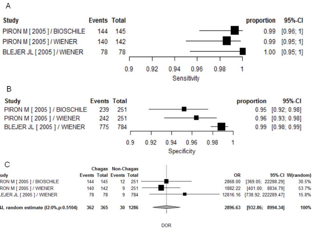
Figure 4 Forest plots of sensitivity (A), specificity (B) and DOR (C) for phase 3 studies investigating commercial ELISA with recombinant antigens. Events - identified as with Chagas disease by the test; OR - (diagnostic) odds ratio; Proportion - sensitivity (or specificity) individual point estimate; Total - number of subject within each sample (with or without Chagas disease); W - weights.
