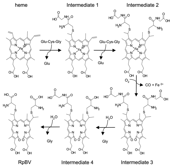
Fig. 4. The proposed heme-degradation pathway in R. prolixus .
