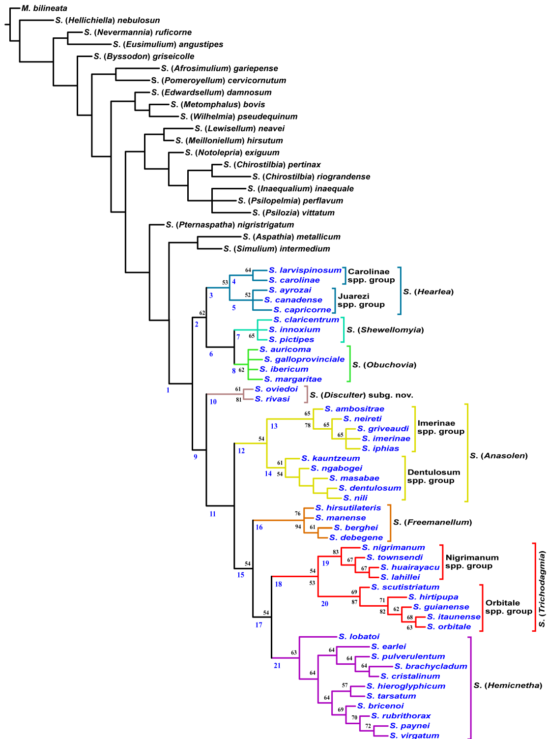
Fig. 1. Strict consensus of the three most parsimonious trees that resulted from the analysis under Implied Weights with K = 3 (Fit = 26.33977; Ci = 0.24; Ri = 0.75). Bremer support values ( > 50 ) mapped above branches and bootstrap values over 50% are given below the nodes. Blue numbers on nodes (1–21) represent clades. Blue terminal taxa are the original ingroup included in the analysis. Colored branches show the proposed classification. Simulium (Disculter) subgen. nov. correspond to old Oviedo species-group.
