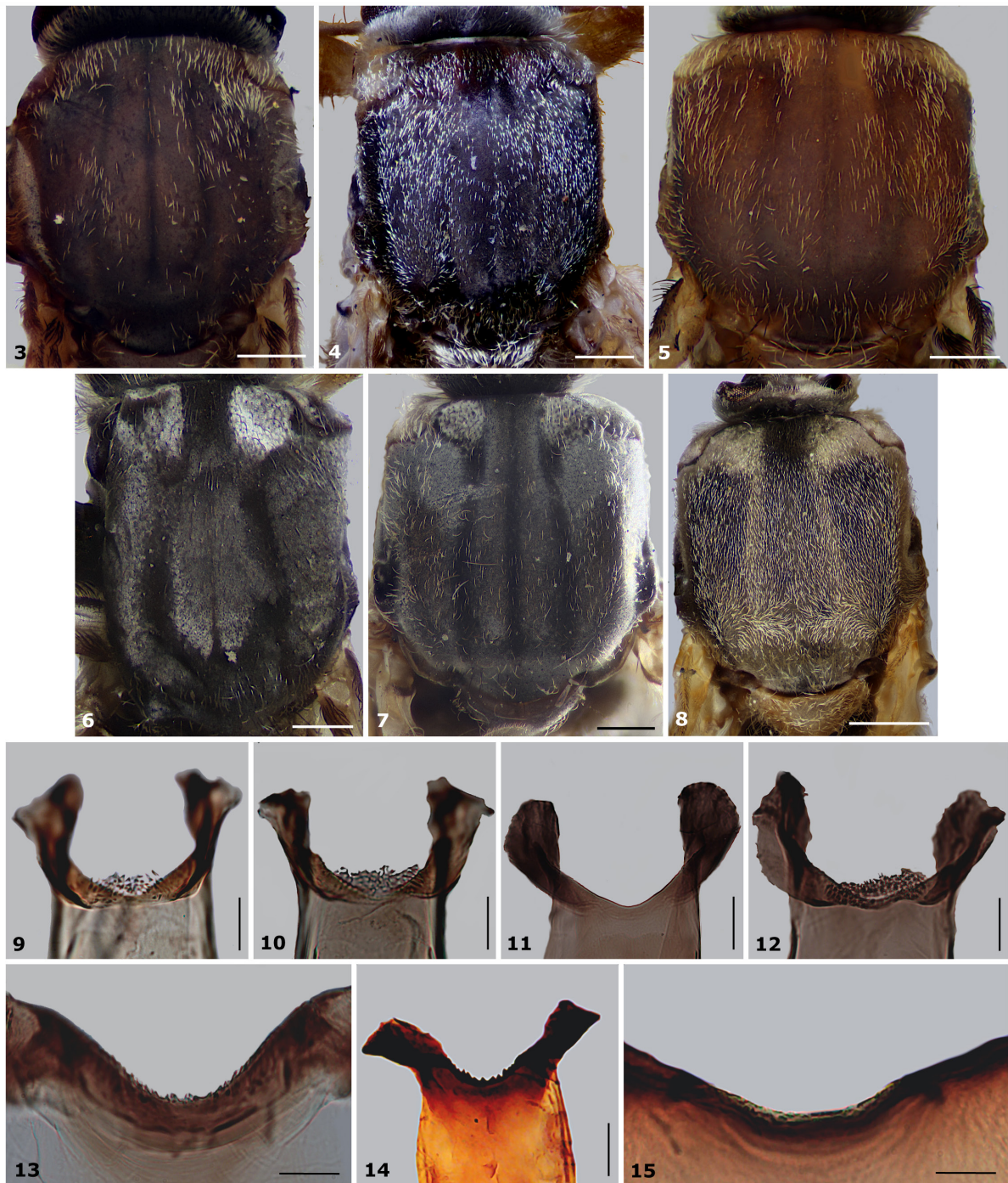
Figs 3–15. Females. 3–8. Thorax, dorsal view. 3–4. Simulium ( Anasolen ) Enderlein, 1930. 3. neireti Roubaud, 1905. 4. nili Gibbins, 1934. — 5. S. ( Freemanellum ) berghei Fain, 1949. — 6. S. ( Hearlea ) canadense Hearle, 1932. — 7. S. ( Shewellomyia ) pictipes Hagen, 1880. — 8. S. ( Obuchovia ) margaritae Rubtsov, 1956. — 9–15. Cibarium of females. 9–12. S. ( Hemicnetha ) Enderlein, 1934. 9. brachycladum Lutz & Pinto, 1932. 10. crystalinum Coscarón & Py-Daniel, 1989. 11. tarsatum Macquart, 1846. 12. pulverulentum Knab, 1915. — 13–15. S. ( Trichodagmia ) Enderlein, 1934. 13. lahillei (Paterson & Shannon, 1927). 14. nigrimanum Macquart, 1838. 15. scutistriatum Lutz, 1909. Scale bars: 3–8 = 0.25 mm; 9–12, 14 = 0.05 mm; 13, 15 = 0.02 mm.
