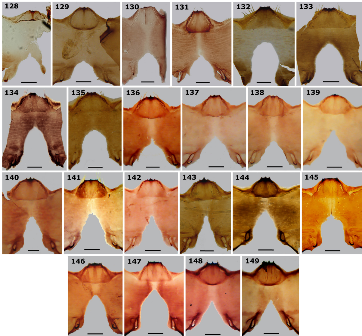
Figs 128–149. Larva (last instar). Postgenal cleft. 128–131. Simulium ( Anasolen ) Enderlein, 1930. 128. ambositrae Grenier & Grjebine, 1959. 129. dentulosum Roubaud, 1915. 130. imerinae Roubaud, 1905. 131. nili Gibbins, 1934. — 132–135. S. ( Freemanellum ) Crosskey, 1969. 132. berghei Fain, 1949. 133. hirsutilateris De-Meillon, 1937. 134. debegene De-Meillon, 1934. 135. manense Elsen & Escaffre, 1976. — 136–139. S. ( Hearlea ) Vargas et al. , 1946. 136. ayrozai Vargas, 1945. 137. canadense Hearle, 1932. 138. capricorne De León, 1945. 139. larvispinosum De León, 1948. — 140–143. S. ( Hemicnetha ) Enderlein, 1934. 140. bricenoi Vargas et al. , 1946. 141. cristalinum Coscarón & Py-Daniel, 1989. 142. paynei Vargas, 1942. 143. rubrithorax Lutz, 1909. — 144. S. ( Obuchovia ) galloprovinciale Giudicelli, 1963. — 145–147. S. ( Trichodagmia ) Enderlein, 1934. 145. hirtipupa Lutz, 1910. 146. lahillei (Paterson & Shannon, 1927). 147. nigrimanum Macquart, 1838. — 148–149. S. ( Disculter ) subgen. nov. 148. oviedo Ramírez-Pérez, 1971. 149. rivasi Ramírez-Pérez, 1971. Scale bars = 0.2 mm.
