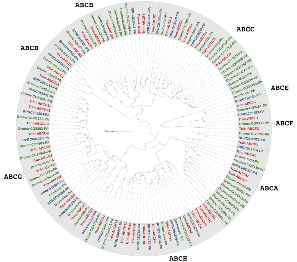
Fig 6. Phylogenetic tree of the ABC transporter superfamily from T. infestans , R. prolixus and D. melanogaster . The maximum-likelihood tree was constructed using IQ-Tree and protein sequences obtained from T. infestans transcriptome (Triin-, red, available in Table G in S2 File) and from R. prolixus (RPRC-, blue, VectorBase ID is shown) and D. melanogaster (Drome-, green, FlyBase gene name and isoform are shown) genomes. Only those sequences complete enough for phylogenetic characterization were included in the tree (remaining sequences were given a preliminary classification shown in brackets in Table G in S2 File). Triatoma infestans sequences were numbered according to their position in the tree. Branches with SH-aLRT support values > 80 are marked with a grey dot. The tree was rooted at midpoint.
