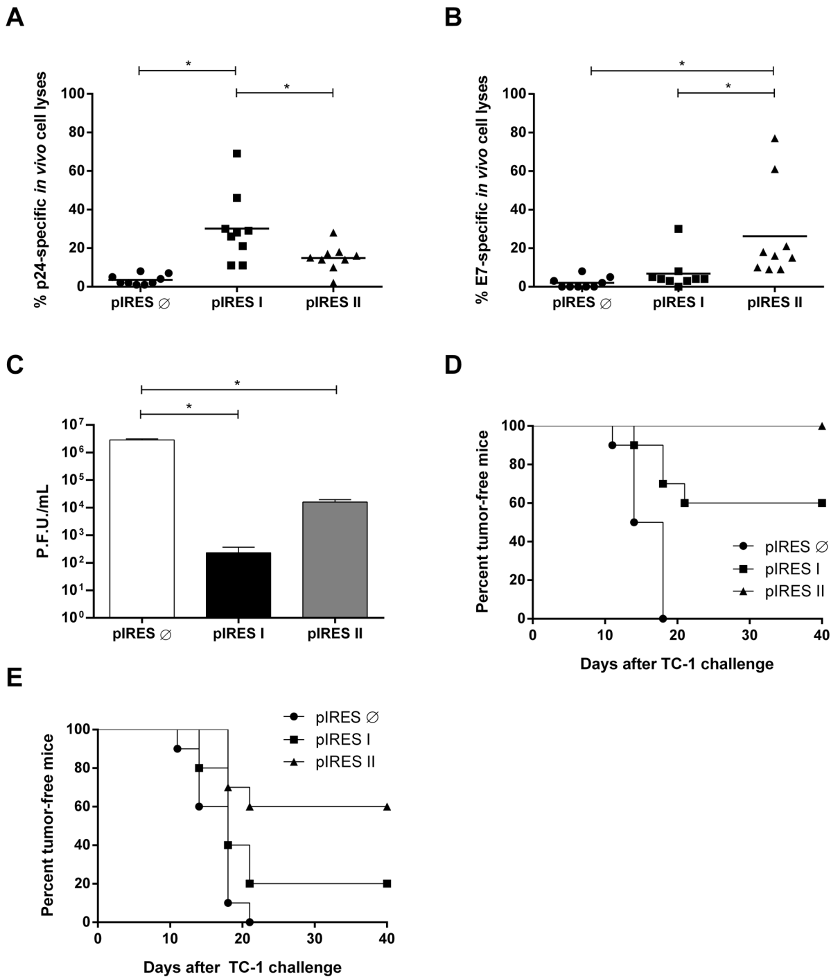
Figure 3. Induction of in vivo E7- and p24-specific cytolytic CD8 + T cell responses in immunized mice. (A–B) In vivo antigen-specific CD8 + T cell-dependent cytotoxic responses in the vaccinated mice was measured two weeks after the last immunization dose. Spleen cells from BALB/c or C57BL/6 mice were labeled with CFSE and pulsed with synthetic peptides representing the immunodominant MHC-I-restricted epitopes of p24 (A) or E7 (B). Data shown in A and B represent the compilation of two independent experiments, encompassing four and five mice per group (n = 9) with results based on the response of each animal. (C) The protective immunity elicited in BALB/c mice immunized with pIRES I or pIRES II was measured after challenge with a recombinant vaccinia virus expressing the HIV-1 protein Gag. Female BALB/c mice were challenged with 2 × 10 6 P.F.U. of rVV-Gag, and 5 days later, the level of viable vaccinia virus in the ovaries was determined after titration in Vero cells. Data shown in C represent the compilation of two independent experiments carried out with pooled samples from five mice per group. *p < 0.05. (D) Prophylactic and (E) therapeutic anti-tumor immunity in C57BL/6 mice immunized with pIRES I or PIRES II. The prophylactic anti-tumor effects were determined in five vaccinated female mice after the s.c. transplantation of 7.5 × 10 4 TC-1 cells two weeks after the last vaccination. The therapeutic anti-tumor effects induced by the vaccines were determined after transplantation of 7.5 × 10 4 TC-1 cells one day before the administration of the first vaccine dose. Data shown in D and E represent the compilation of two independent experiments, with five mice per group. The survival curves D and E raised p values of 0.0001 and 0.0006, respectively, in the Logrank test for trend. pIRES is the empty vector used as immunization control. doi:10.1371/journal.pone.0071322.g003
