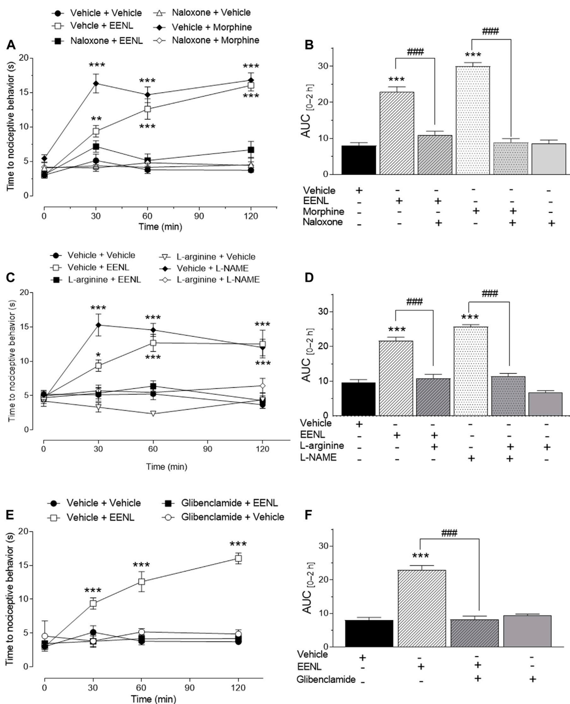
FIGURE 6 Pharmacological interpretation of the effect of EENL in the hot plate test. The effect of the opioid system (A, B), L-arginine/nitric oxide pathway (C, D), and ATP-sensitive K + channel inhibitors (panels E and F) was verified in the antinociception caused by EENL. Each value represents the mean ± SEM of n = 5–6. (A, C, E) Two-way ANOVA followed by the Tukey post-test; *p < 0.05, **p < 0.01 or ***p < 0.001 vs. respective vehicle-treated group. (B, D, F) One-way ANOVA followed by the Tukey post-test. ***p < 0.001 vs. vehicle and ###p < 0.001.
