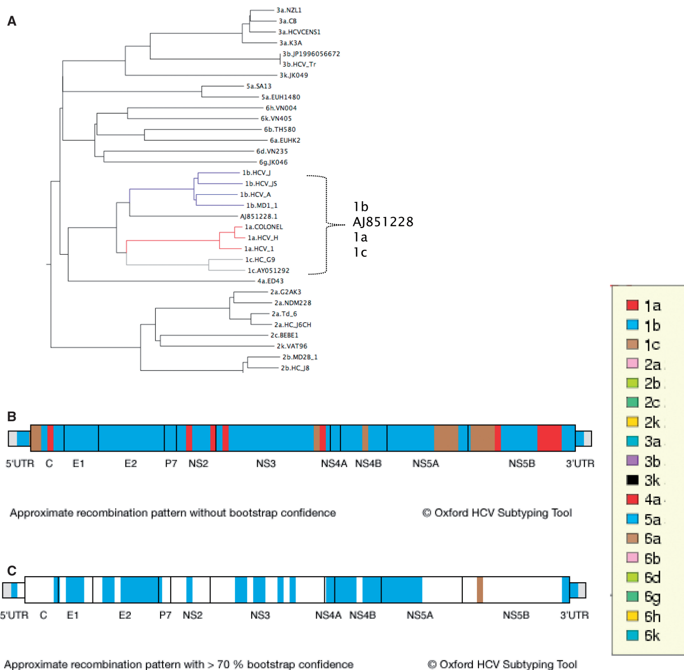
Figure 2. (A) Phylogenetic tree showing the location of the AJ851228 sequence. (B) Recombination profile without bootstrap confidence (top panel); recombination profile with >70% bootstrap confidence.
