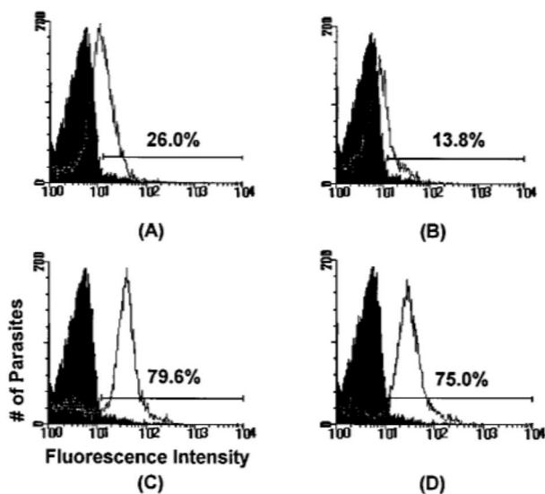
FIG. 4. Histograms representing PFPF before (A and C) and after (B and D) the SYNSORB 115 absorbing assay. Each panel presents the results of an overlay FLI histogram by using the test serum (blank area) and the FITC-conjugated anti-human IgG control (solid area). The PFPF of a serum sample from a DIS patient (A) changed after the use of a SYNSORB 115 column (B), whereas the PFPF of a serum sample from an NT patient (C) did not change (D). This result confirms the expectation that detection of MBA in that particular serum sample from a DIS patient was due to cross-reactive galactosyl-protein epitopes, as previously reported (6), and can be abolished by absorption.
