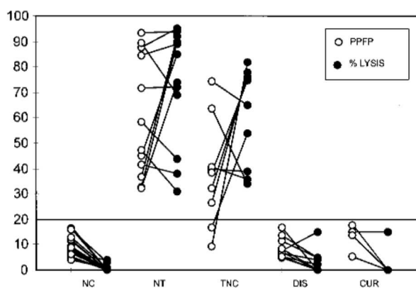
FIG. 5. Scatter graphs showing PFPF and percent lysis ranges for the groups analyzed. For comparative analysis, the PFPF and percent lysis for each serum sample tested are indicated by connecting lines. Using 20% as a cutoff between effective and ineffective treatment, we identified that all NT patients could be distinguished from both DIS and CUR patients as well as from NC individuals. However, two TNC patients fell below the cutoff.
