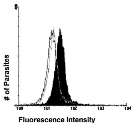
FIG. 3. FLI histograms representing the mean pattern of fluorescent parasite distribution obtained with sera from treated patients. The histogram profile of serum from a DIS patient totally overlaps the profile of serum from a CUR patient, whereas serum from a TNC patient differs from the others, showing minimal overlapping and with the peak located in the positive region of the graph. According to the data, sera from patients with active infection following specific treatment could be distinguished from both DIS and CUR patients. These results reemphasize that MBA searching is a useful tool to monitor the effectiveness of treatment of Chagas' disease.
