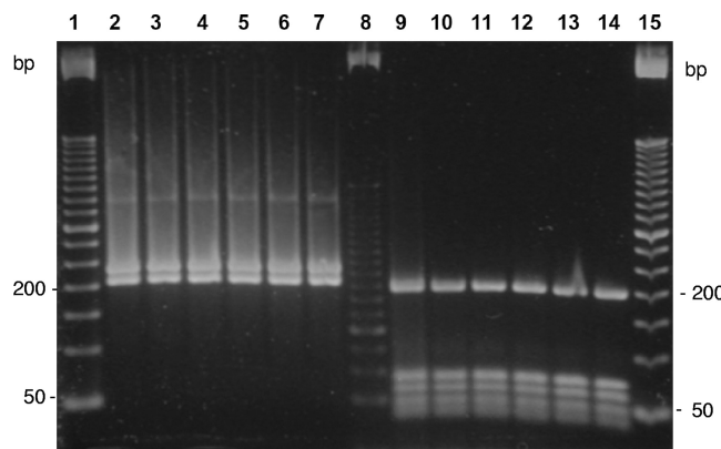
FIG. 2. PRA- hsp65 profiles of six representative M. massiliense epidemic isolates. Lanes 1 and 15, 50-bp DNA ladder; lane 8, 25-bp DNA ladder; lanes 2 to 7, amplicons digested with BstEII; lanes 9 to 14, amplicons digested with HaeIII. Each lane represents a different strain: lane 2, CRM-0006; 3, CRM-0018; 4, CRM-0029; 5, CRM-0181; 6, CRM-0189; 7, CRM-0195; 9, CRM-0006; 10, CRM-0018; 11, CRM-0029; 12, CRM-0181; 13, CRM-0189; and 14, CRM-0195.
