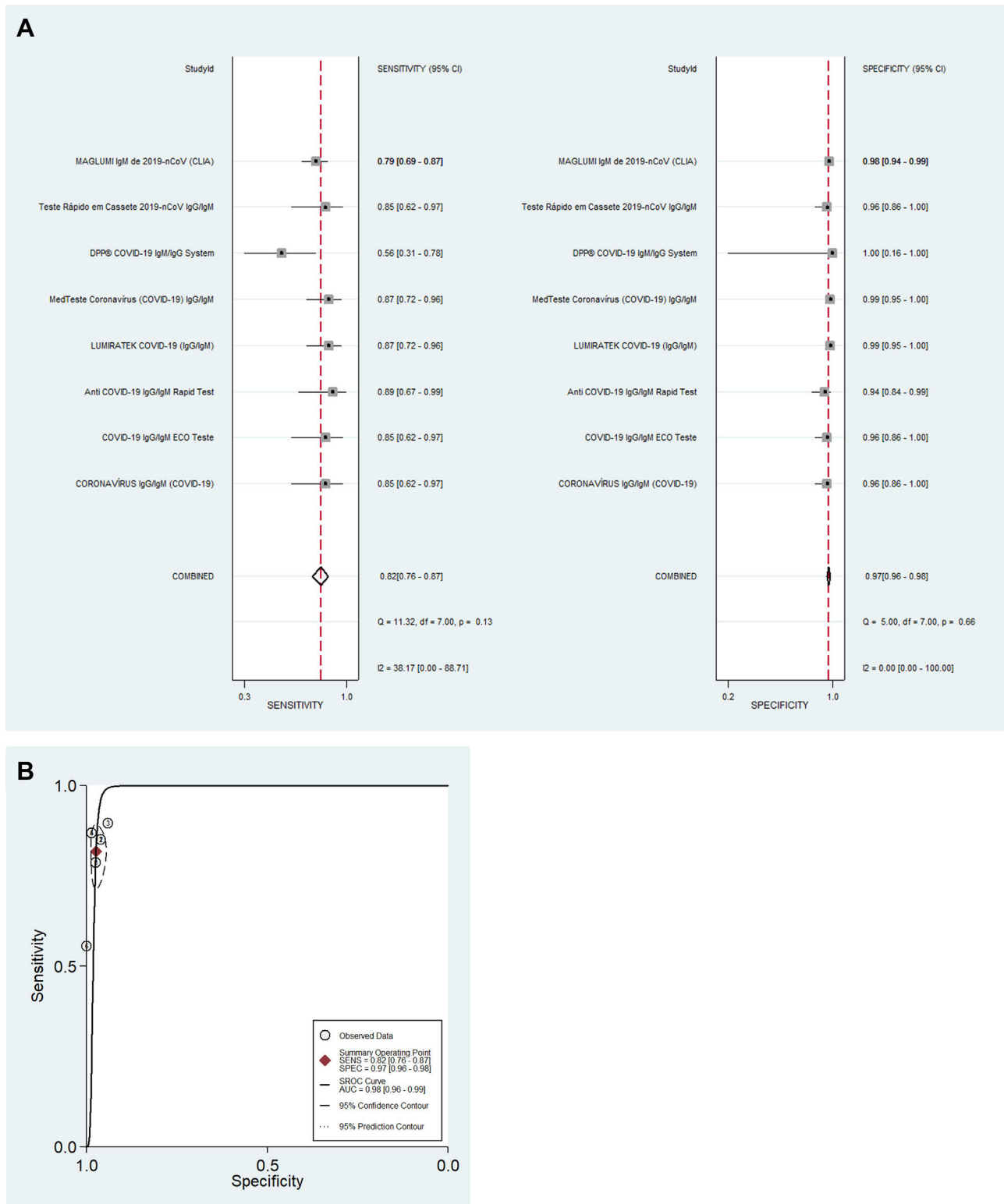
Fig. 1 – Pooled diagnostic accuracy analysis (A) and summary receiver operating characteristic curve (B) of tests (n = 8) for detection of IgM antibodies tests against SARS-CoV-2.
