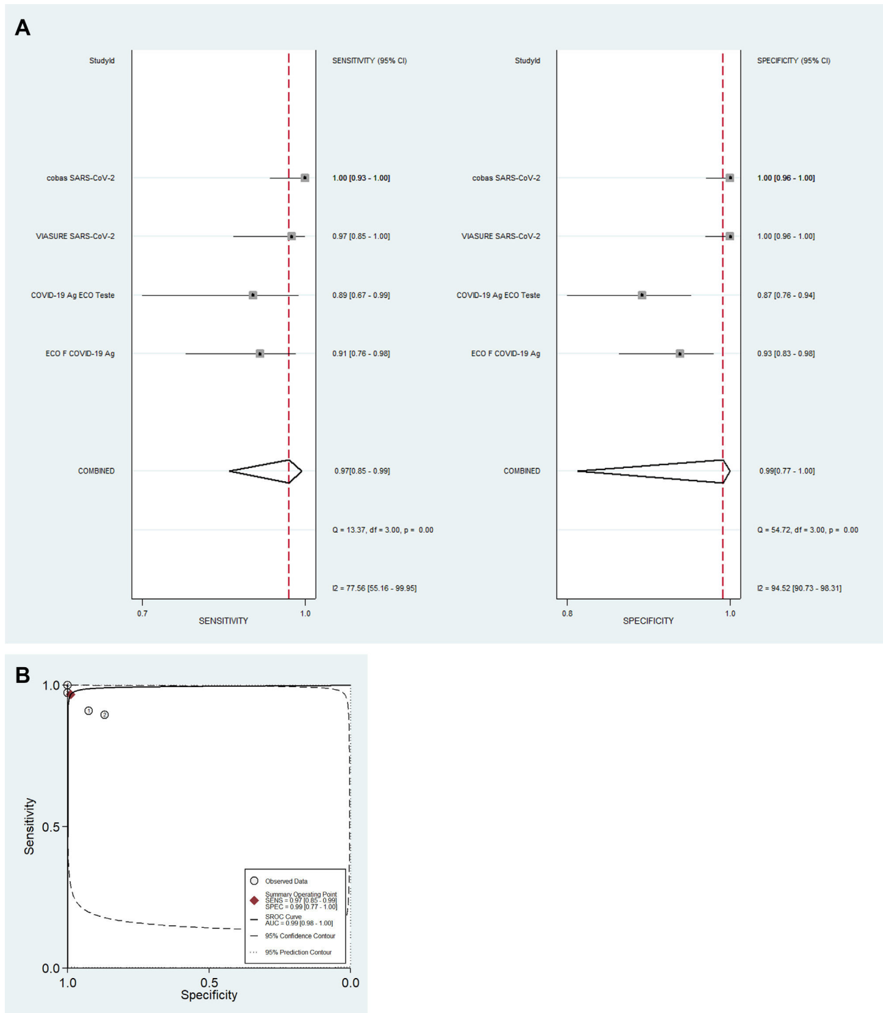
Fig. 3 – Pooled diagnostic accuracy analysis (A) and summary receiver operating characteristic curve (B) of tests (n = 4) using nasopharyngeal and/or oropharyngeal swabs for detection of antigen or nucleic acid of SARS-CoV-2.
