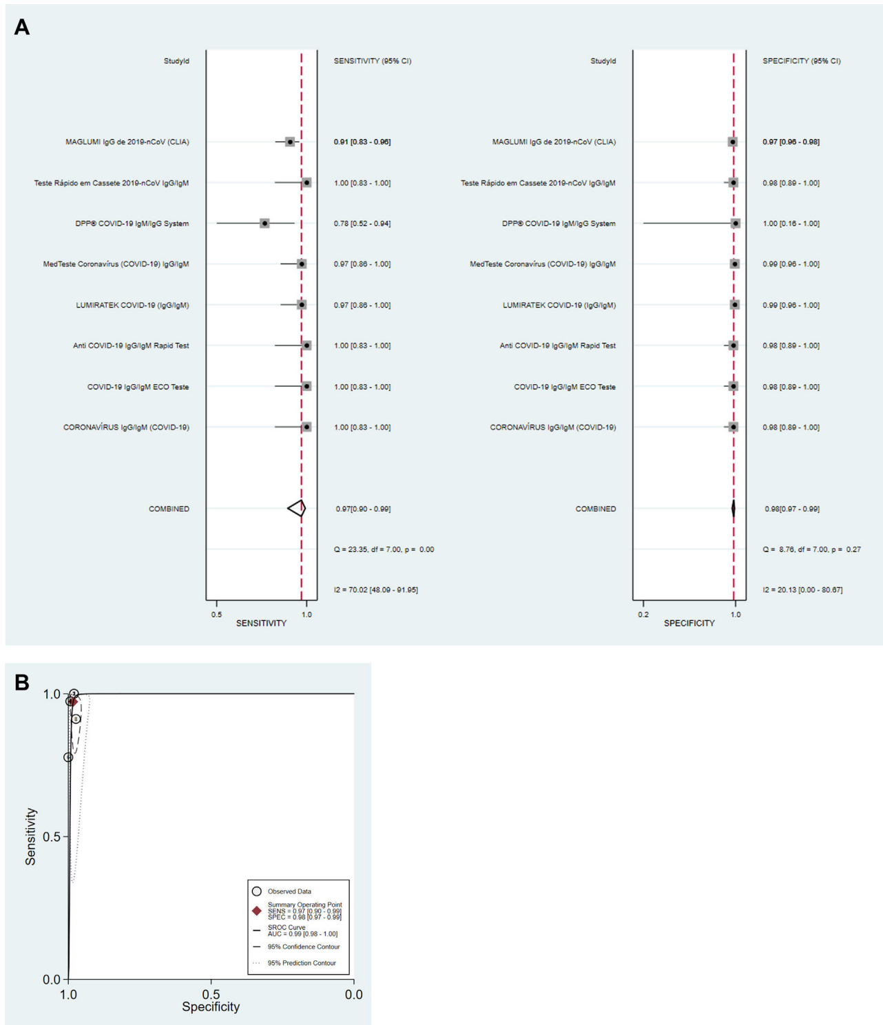
Fig. 2 – Pooled diagnostic accuracy analysis (A) and summary receiver operating characteristic curve (B) of tests (n = 8) for detection of IgG antibodies tests against SARS-CoV-2.
