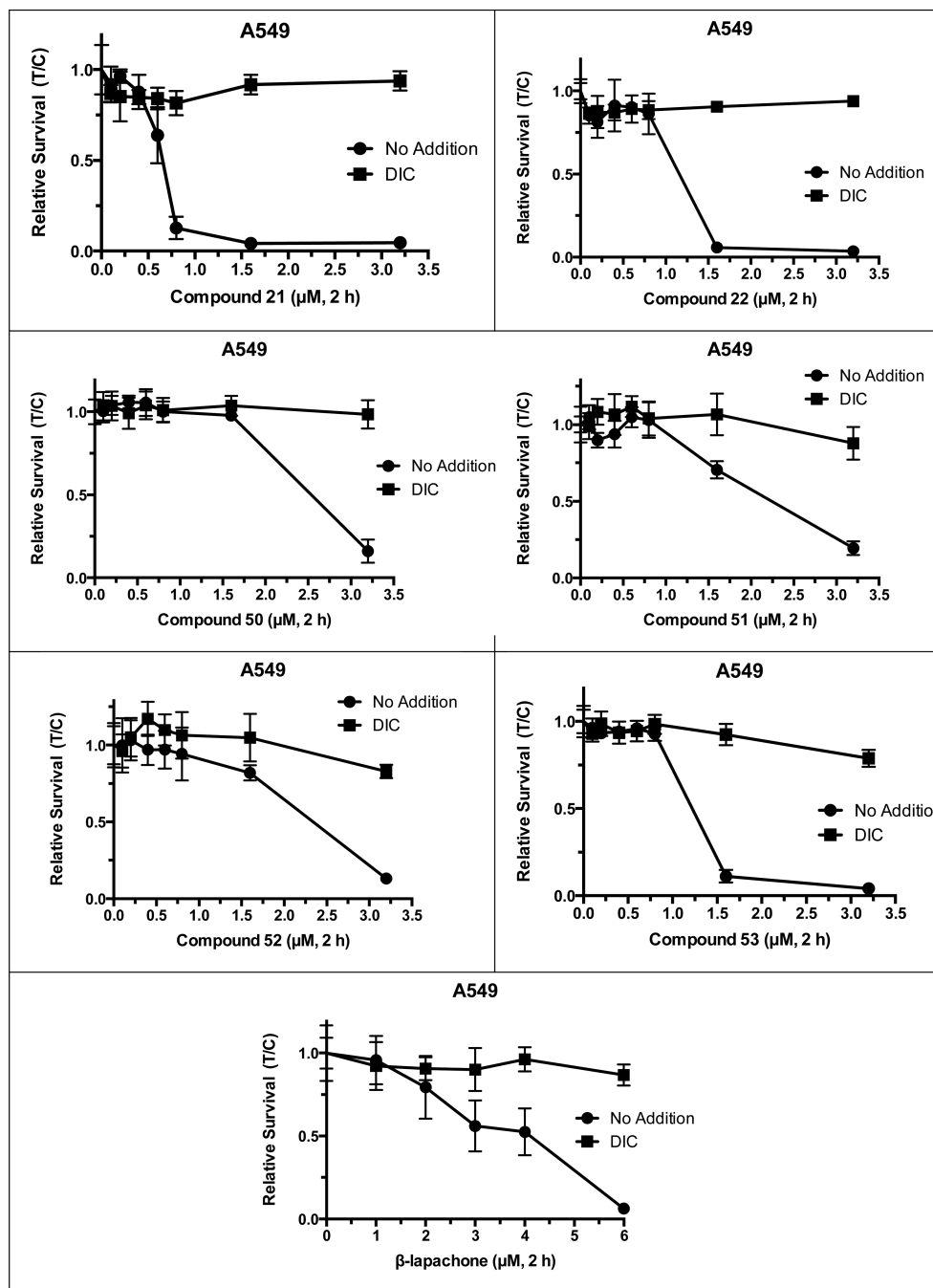
Figure 2. Compounds 21, 22, 50-53 and β-lapachone evaluated for NQO1-dependence.
