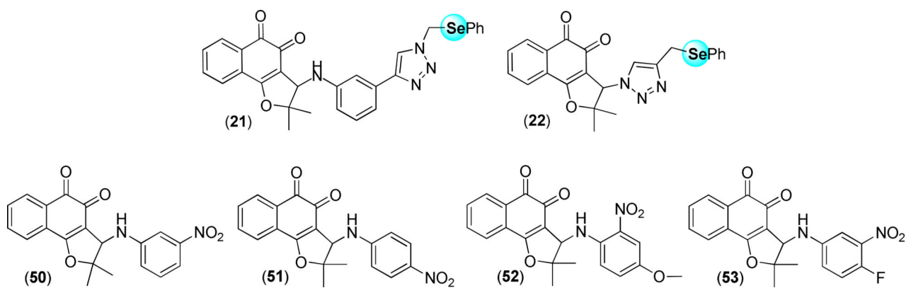
Figure 1. Selected compounds for NQO1- and GPx-specific studies.
