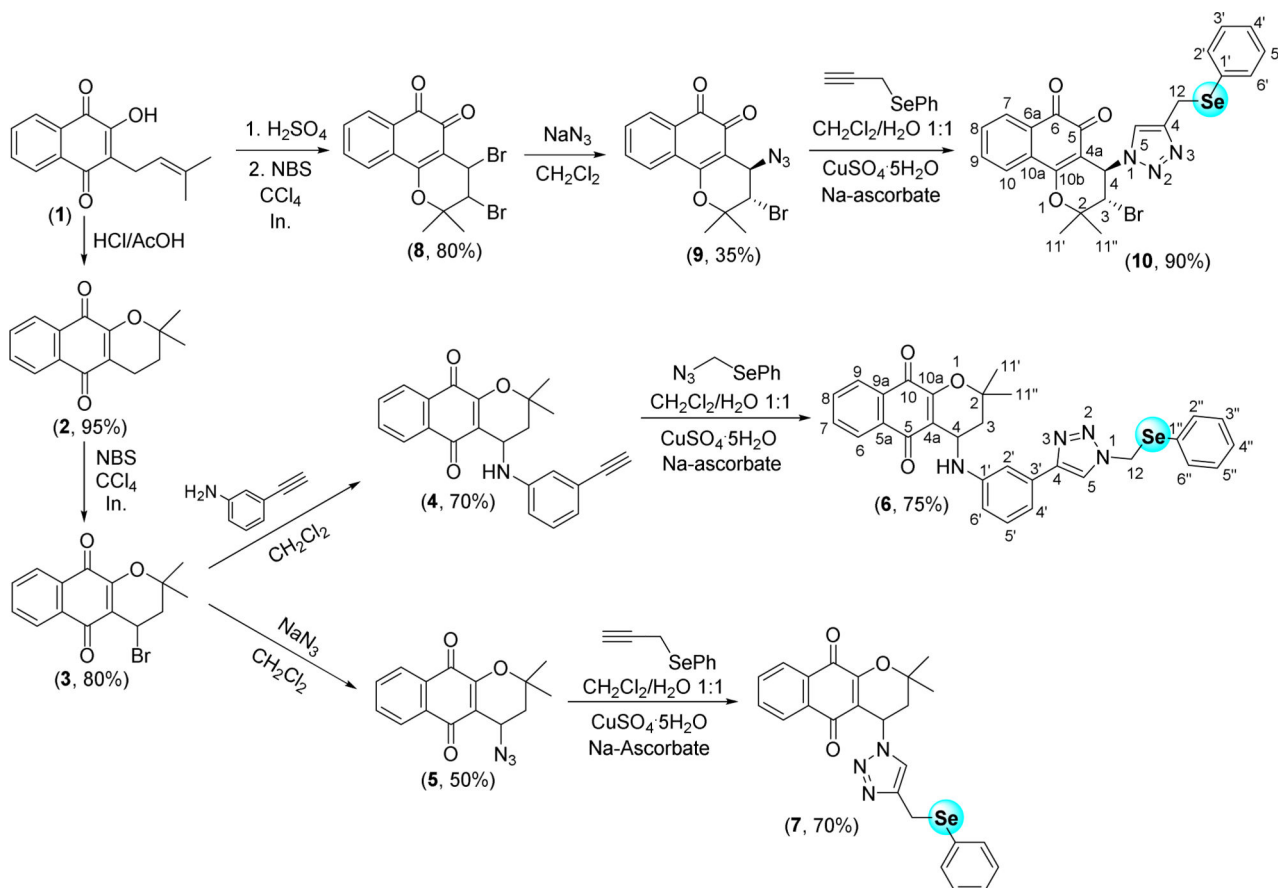
Scheme 2. Synthesis of selenium-containing \beta -lapachone and \alpha -lapachone-based 1,2,3-triazoles.
