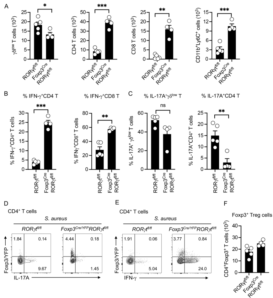
Figure S3. ROR \gamma t + Foxp3 + Treg cells control the IFN- \gamma -producing CD4 and CD8 T cells. (A) Absolute cell numbers of \gamma\delta^{\text{low}} T, CD4 T, and CD8 T cells and monocytes in the skin of S. aureus -colonized RORγt fl/fl and Foxp3 Cre RORγt fl/fl mice on day 10. Mean \pm SEM representative of two experiments with four to five mice per group. (B) Percent of IFN- \gamma + CD4 + T and IFN- \gamma + CD8 + T cells in the skin of S. aureus -colonized RORγt fl/fl and Foxp3 Cre RORγt fl/fl mice at day 10 by flow cytometry. Mean \pm SEM representative of two experiments with four to five mice per group. (C) Percent of IL-17A + \gamma\delta^{\text{low}} T and IL-17A + CD4 + T cells in the skin of S. aureus -colonized RORγt fl/fl and Foxp3 Cre RORγt fl/fl mice at day 10 by flow cytometry. Mean \pm SEM representative of two experiments with four to five mice per group. (D and E) Flow cytometry analysis of Foxp3 YFP and IL-17A and IFN- \gamma in CD4 + T cells in S. aureus -colonized RORγt fl/fl and Foxp3 Cre /YFP/RORγt fl/fl mice at day 10. Representative of two experiments with four mice per group. Numbers in contour plots indicate the percent of cells within the gates. (F) Absolute cell numbers of Foxp3 + Treg cells in S. aureus -colonized RORγt fl/fl and Foxp3 Cre RORγt fl/fl mice at day 10. Mean \pm SEM representative of one experiment with four to five mice per group. *P < 0.05, **P < 0.01, and ***P < 0.001. "ns" denotes not significant. Significant P values by two-tailed unpaired Student's t test with Welch's correction are indicated in the figure.
