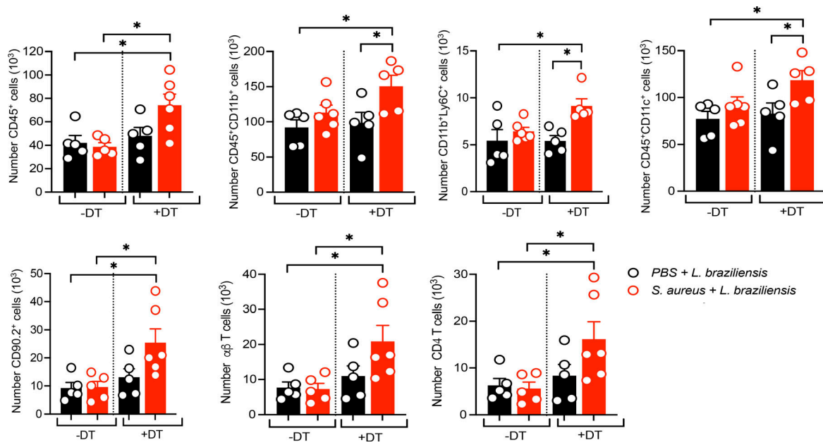
Figure S4. Impact of reduced Foxp3 + Tregs in S. aureus -colonized and L. braziliensis -infected mice. Foxp3-DTR heterozygous female mice were colonized on day 1-, and then at day 10 (week 0) mice were infected with L. braziliensis in one ear as in Fig.2A and euthanized at week 6 for analysis. Mice treated with DT at weeks 0, 1, 2, 3, 4, and 5 to chronically reduce the Foxp3 + Tregs. Absolute numbers of CD45 + , CD45 + CD11b + , CD11b + Ly6C + , CD45 + CD11c + , CD90.2 + , αβ T cells, and CD4 T cells in the ear skin of different treatment groups of treated (+DT) and untreated (-DT) with DT at week 6. Mean ± SEM representative of one experiment with five to six mice per group. *P < 0.05. Significant P values by two-tailed unpaired Student's t test with Welch's correction are indicated in the figure.
