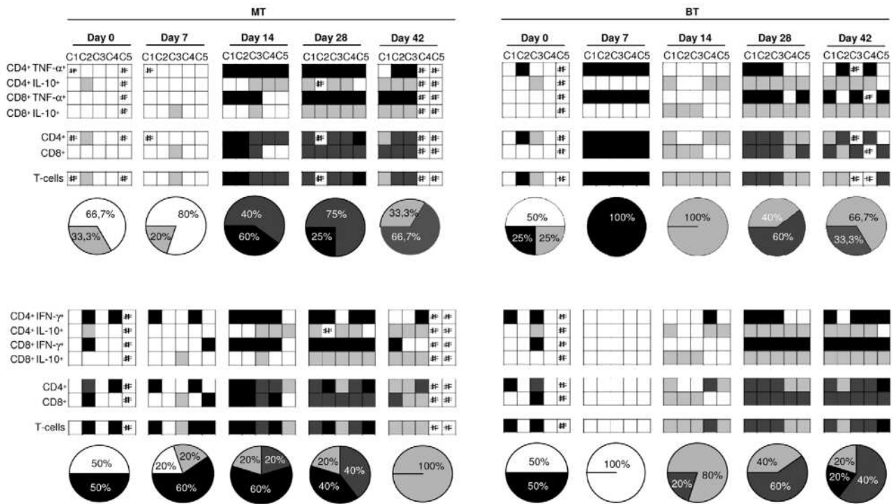
Figure 5. Cytokine profile of spleen T-lymphocytes from mice before (0) and at 7, 14, 28 and 42 days after infection with metacyclic (MT) or blood trypomastigotes (BT) of Trypanosoma cruzi . "Gray scale" diagrams were used to represent the cytokine pattern and the cytokine balance within T-cell subsets besides the overall cytokine balance with T-cells, highlighting the predominance of "low" cytokine-producers (white square), "high" TNF- \alpha or IFN- \gamma producers (black square), "high" IL-10 + producers (light gray square) or "high" mixed cytokine-producers (dark gray square). Pie charts represent the percentage of animals displaying a given T-cells overall cytokine balance selectively amongst the "high" cytokine-producers. ND = Not detected.
