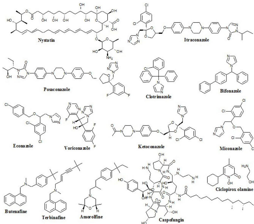
Figure 4. Antifungal drugs
