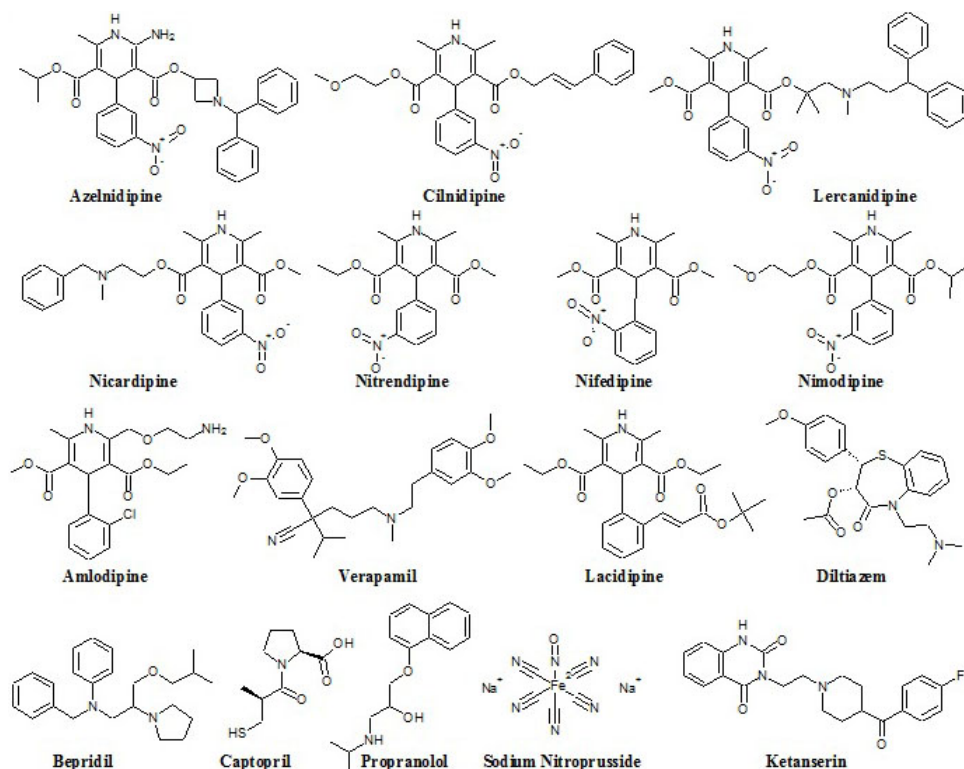
Figure 8. Antihypertensive drugs
