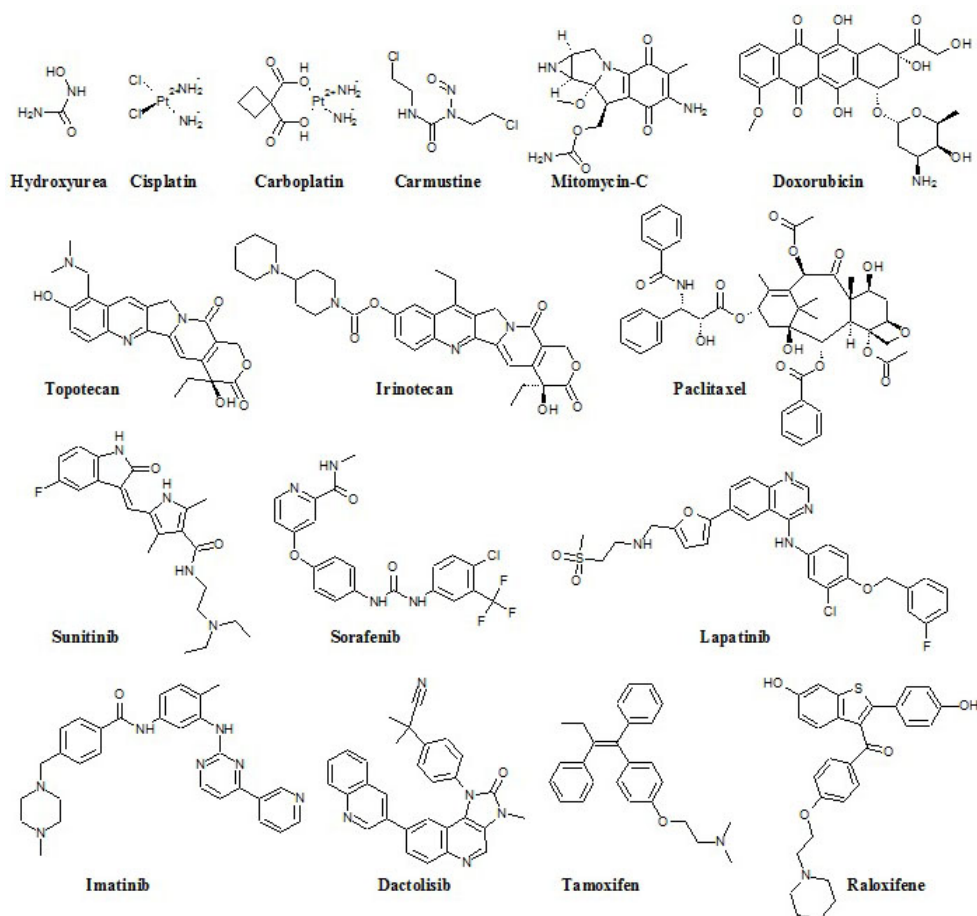
Figure 6. Anticancer drugs
