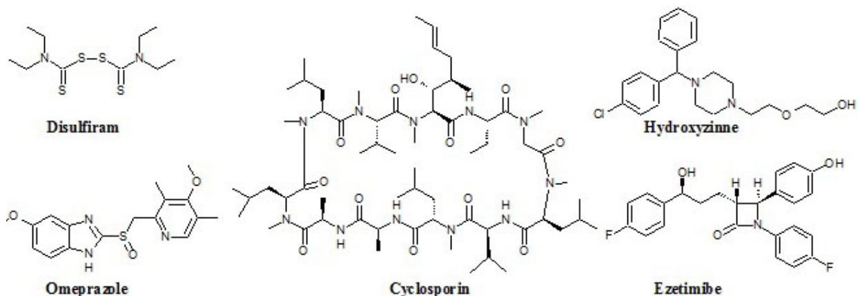
Figure 10. Miscellaneous drugs
